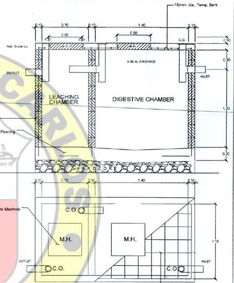
DETAILS OF SEPTIC VAULT SCALE: 1:25 MTS
